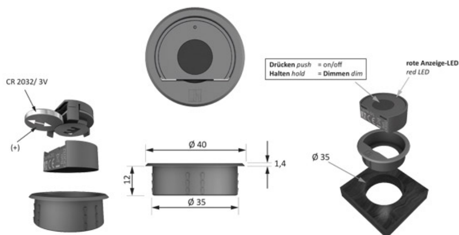
31.108.01 / 31.109.01 Smartempfänger smartreceiver 12VDC / 24VDC
